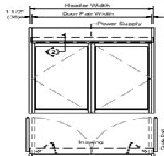
Pair Unit Floor Plan with Elevation LHR-RHL shown. LHR-RHR is Outswing
