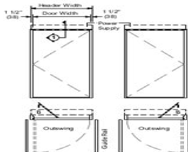
Single Units Floor Plans with Elevations LHR & RHR shown. LH & RH are Inswing
