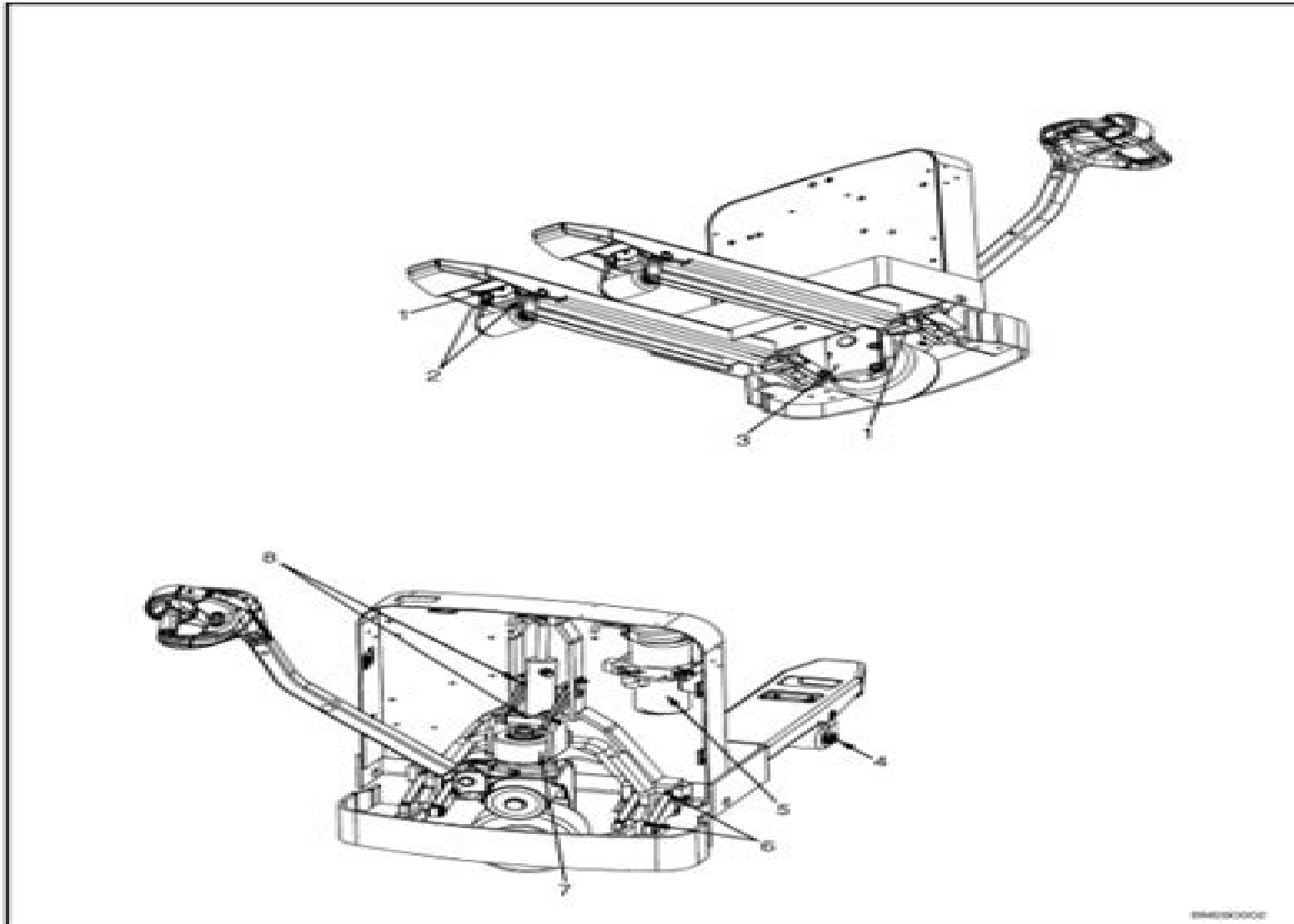
Figure 8. Lubrication Locations
