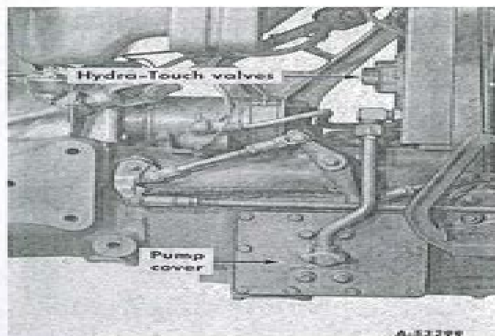
Illust. 45B Left side of Hydra-Touch system with internal pump.
