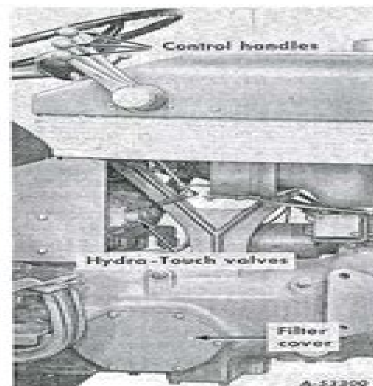
Illust. 45C Right side of Hydra-Touch system with internal pump.
