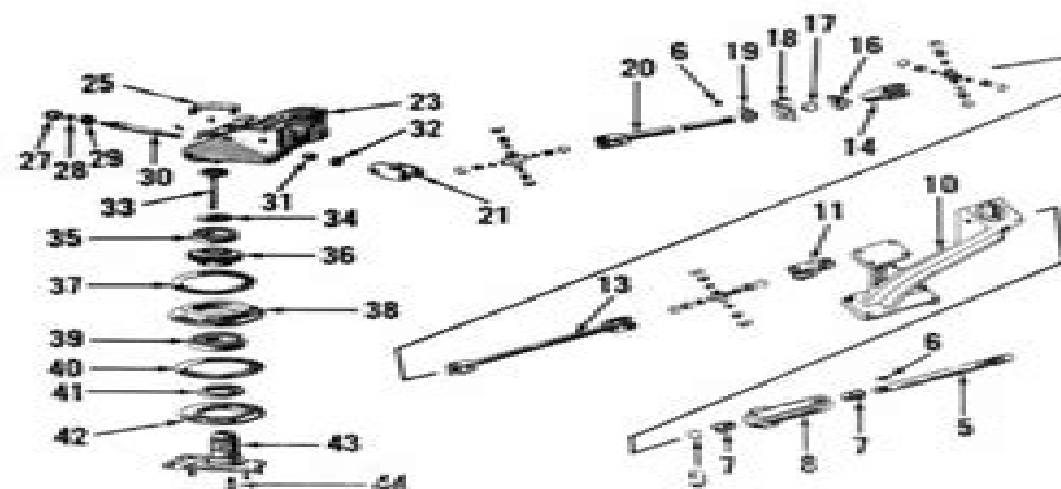
Fig. 1H13-05—Exploded view of the manual steering gear unit used on Farmall 340 tractors. Farmall 504 tractors are basically similar.
