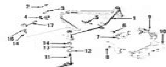
Fig. IH1304—Exploded view of the non-adjustable front axle which is available on 330 and 340 International tractors. Except for front bolsters and brackets, series 504 and 2504 International tractors are similar. Refer to Fig. IH1303 for legend.
