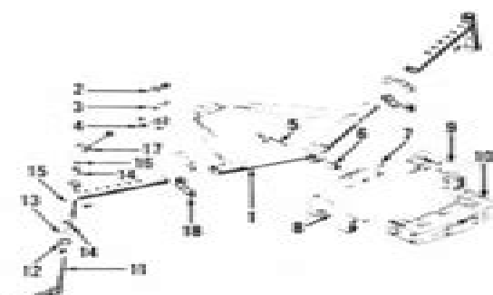
Fig. IH1303 —Exploded view of the adjustable front axle which is available on 330 and 340 International tractors. Except for front bolster and brackets, series 504 International tractors are similar.
