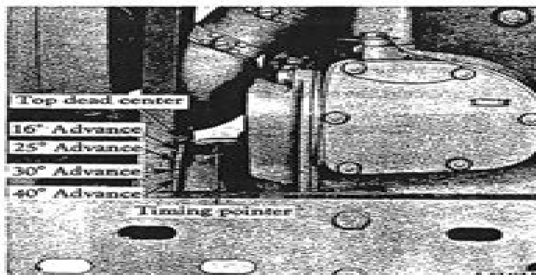
Illustr. 10 Timing pointer.
