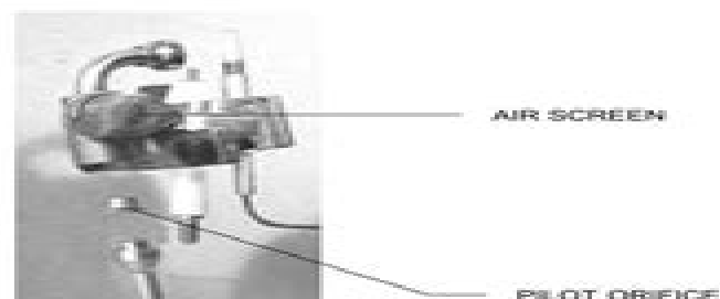
Fig. 10 - Pilot burner with air screen/ pilot orifice
