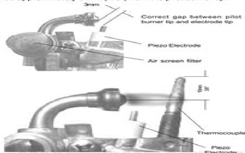
Fig. 9 - Characteristic Pilot Flame
