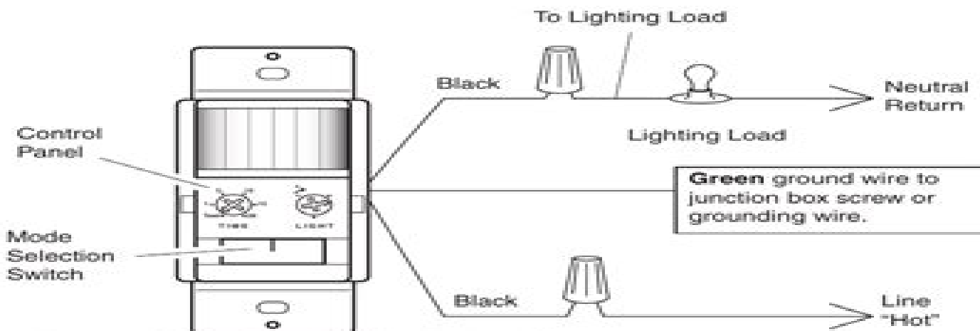
Figure 3 - Connecting Electrical Leads of Sensor
