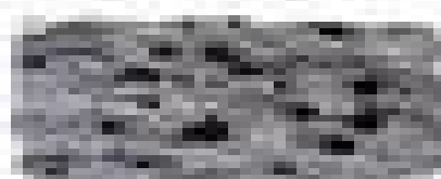
Basaltic rock Photomicrograph of a basaltic rock
