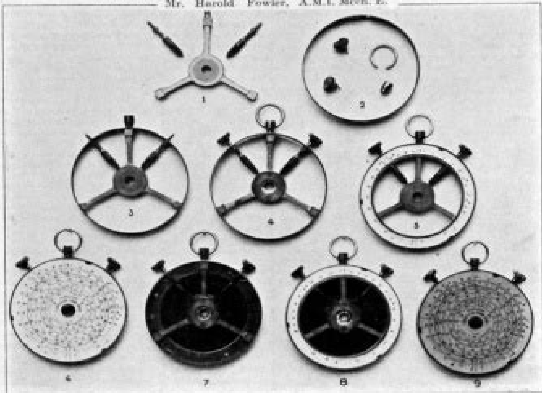
FOWLER'S CIRCULAR SLIDE RULE CALCULATOR
