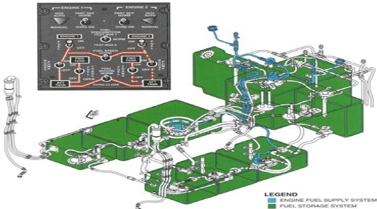
Figure 5B-1. Airframe Fuel System
