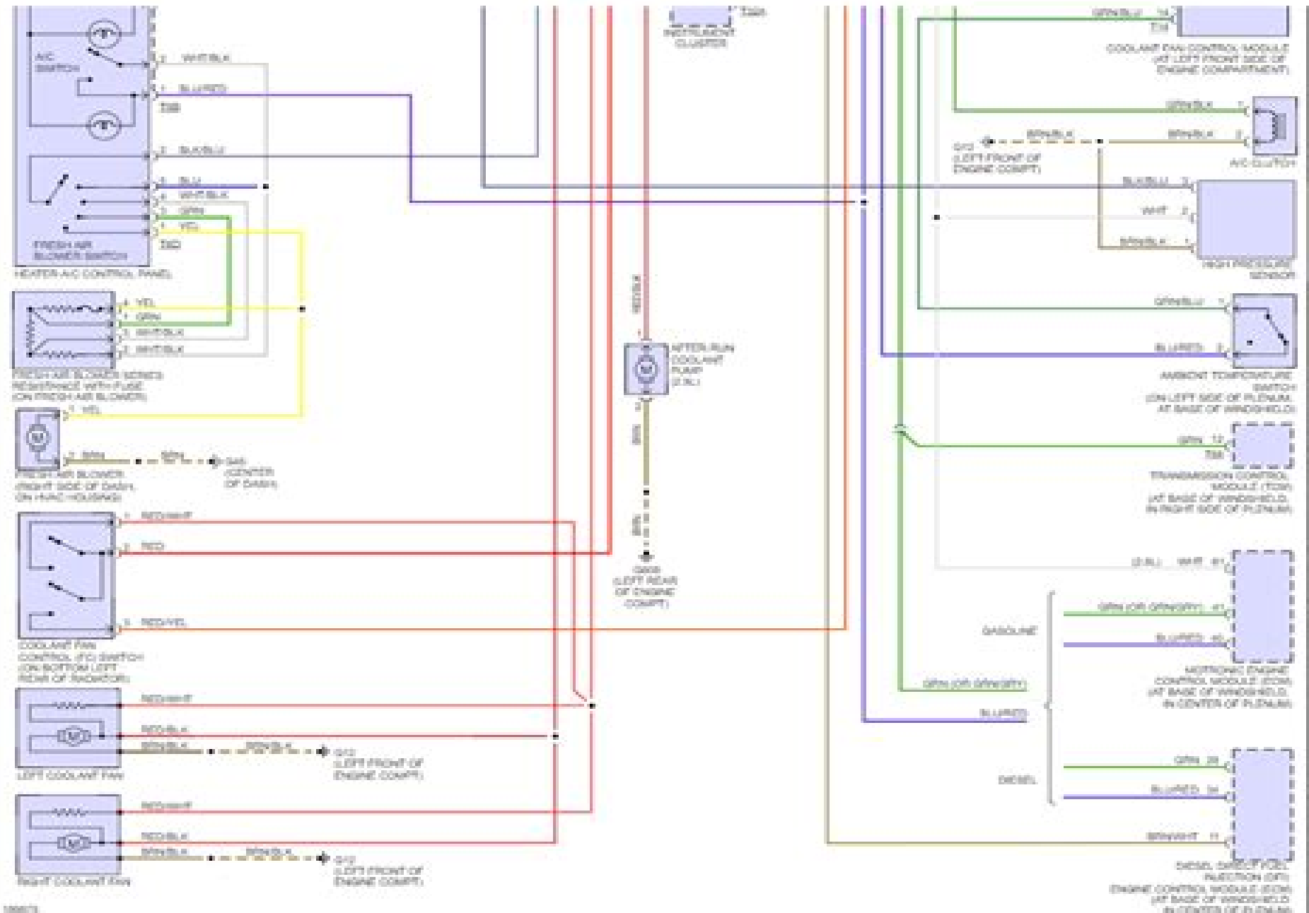
Fig 1: Manual A/C Circuit
