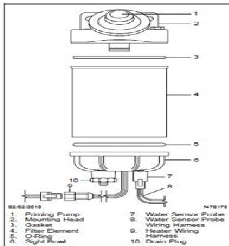
Fig. 1, Fuel/Water Separator Assembly
