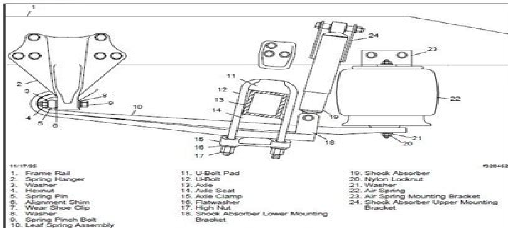
Fig. 1, Rear Axle Suspension
