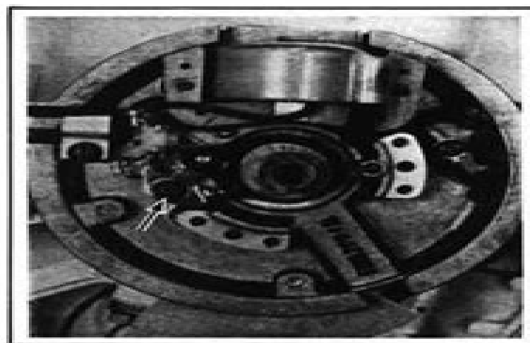
Figure 3. Removing Condenser.
