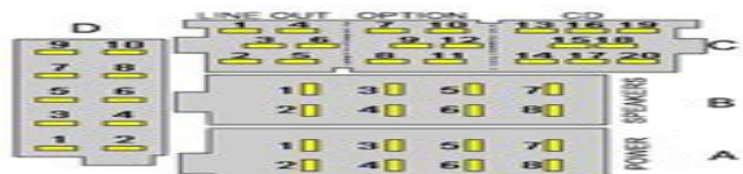
46 (5+8+10+20) pin ISO 10487 Head Unit / Car Stereo connector
