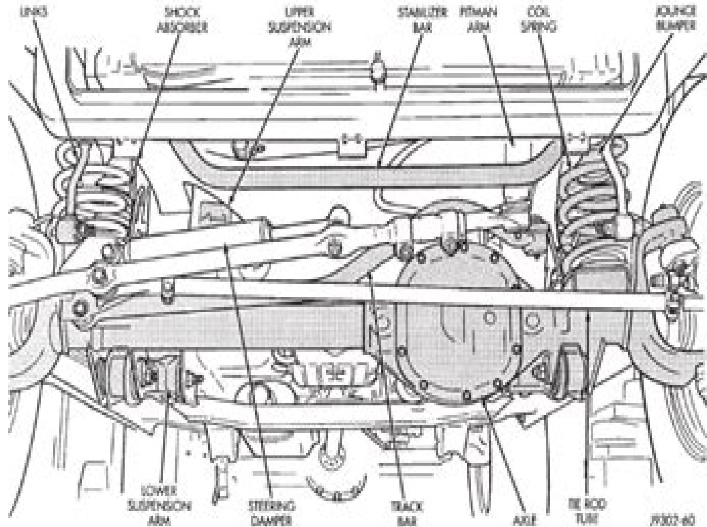
Fig. 1 Front Suspension
