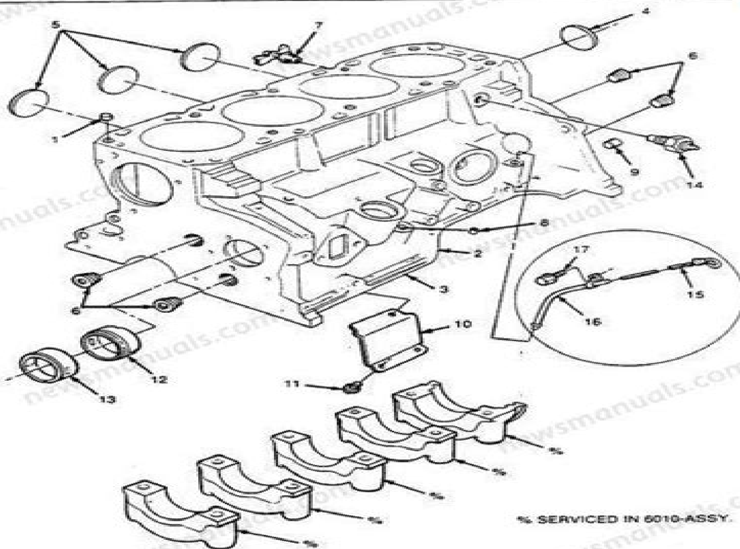
CYLINDER BLOCK AND RELATED PARTS — TYPICAL
