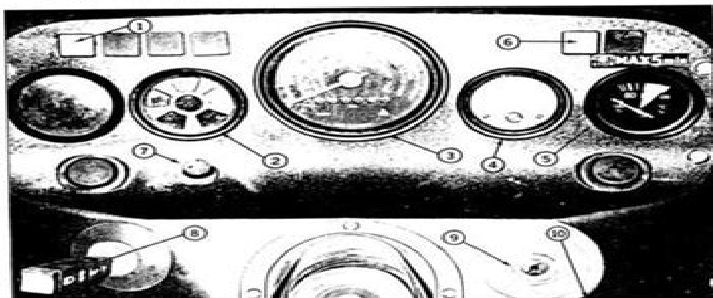
Figure 3. Dashboard: 1) directional signal, 2) warning lights cluster, 3) speedometer and PTO shaft rpm, 4) fuel gauge, 5) coolant temperature gauge, 6) PTO shaft clutch indicator, 7) rear working light switch, 8) high beam, directional signal, and horn lever, 9) ignition switch key, 10) starter pushbutton - see figure 16.
