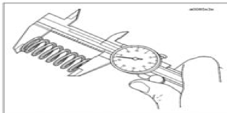
Figure 3-56. Checking Spring Free Length
