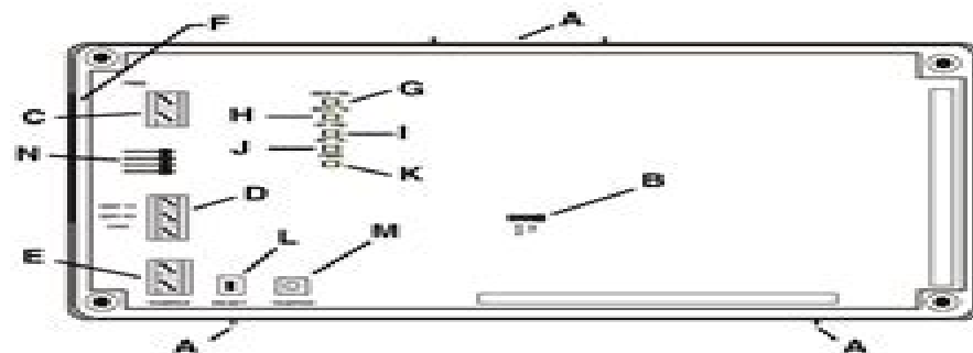
Figure 1 Network Coordinator components
