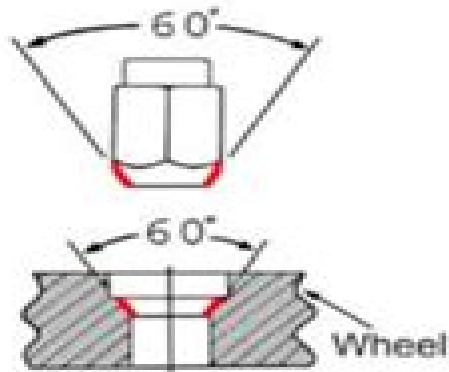
Acorn/Tapered Cone Seat
