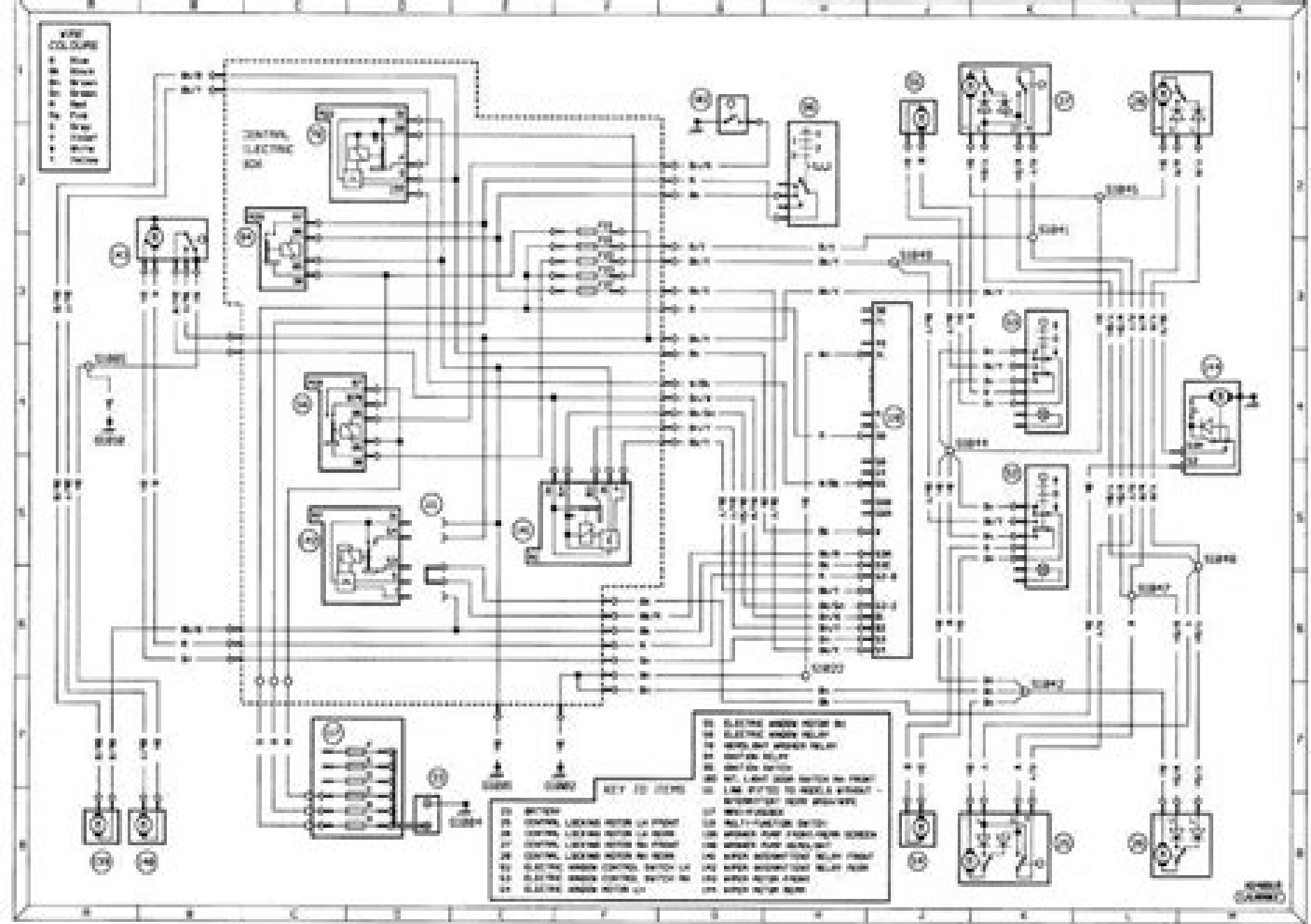
Diagram 12: Typical wash/wipe, central locking and electric windows
