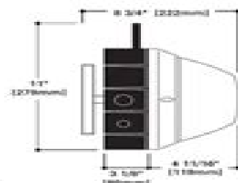
SIDE DIMENSIONS
