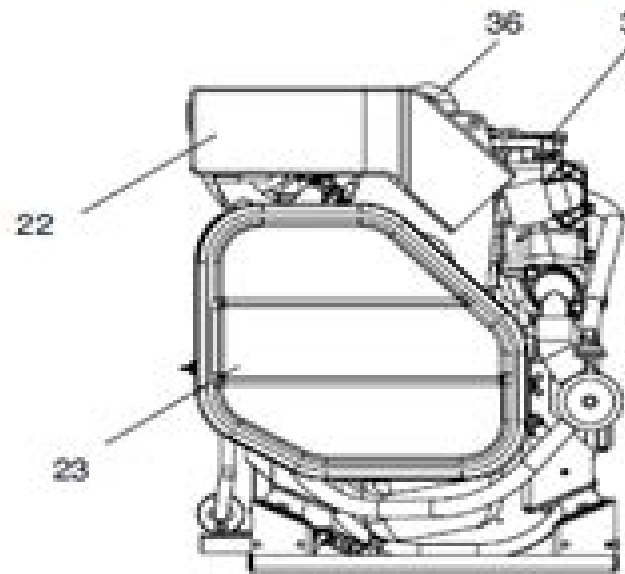
ENGINE-END VIEW
