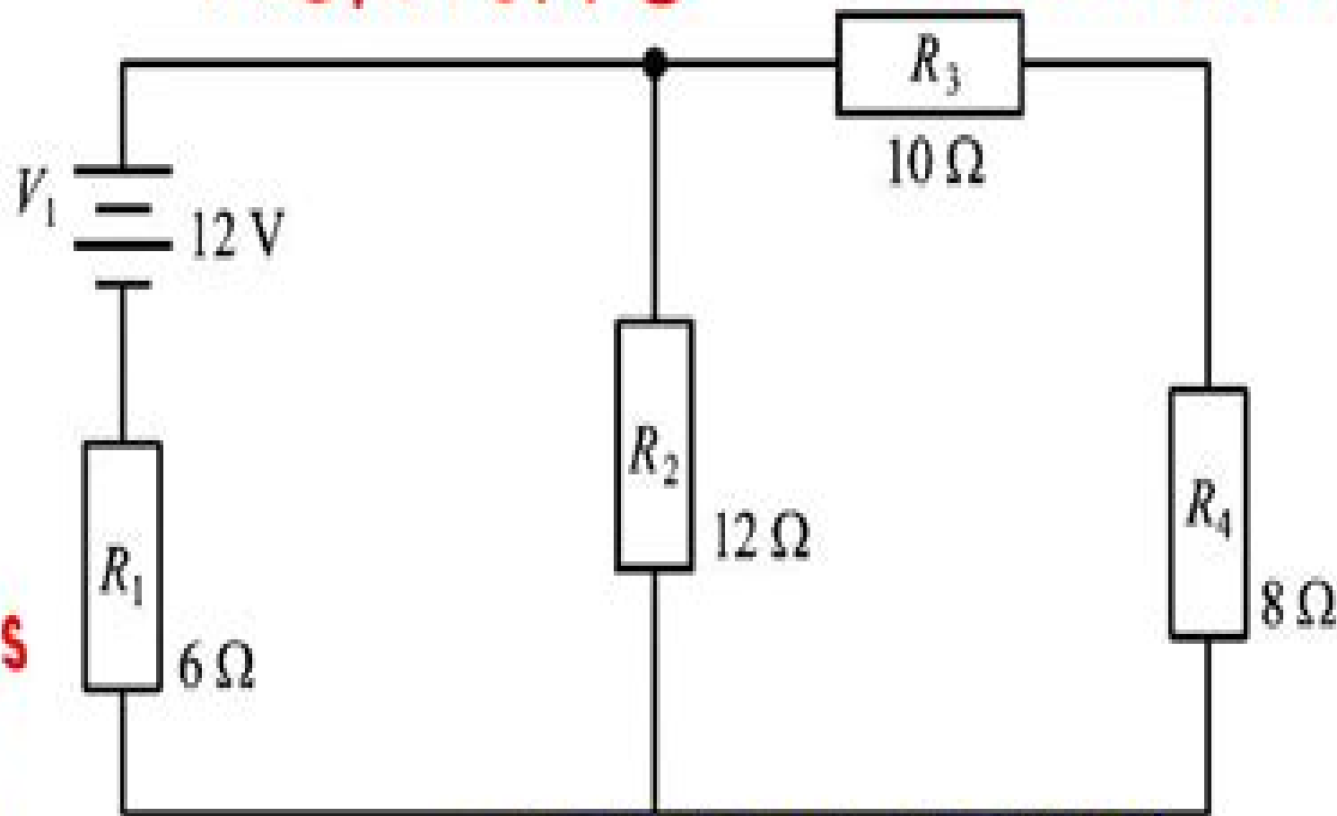
Figure 1.23(a): Circuit with four resistors and one voltage source
