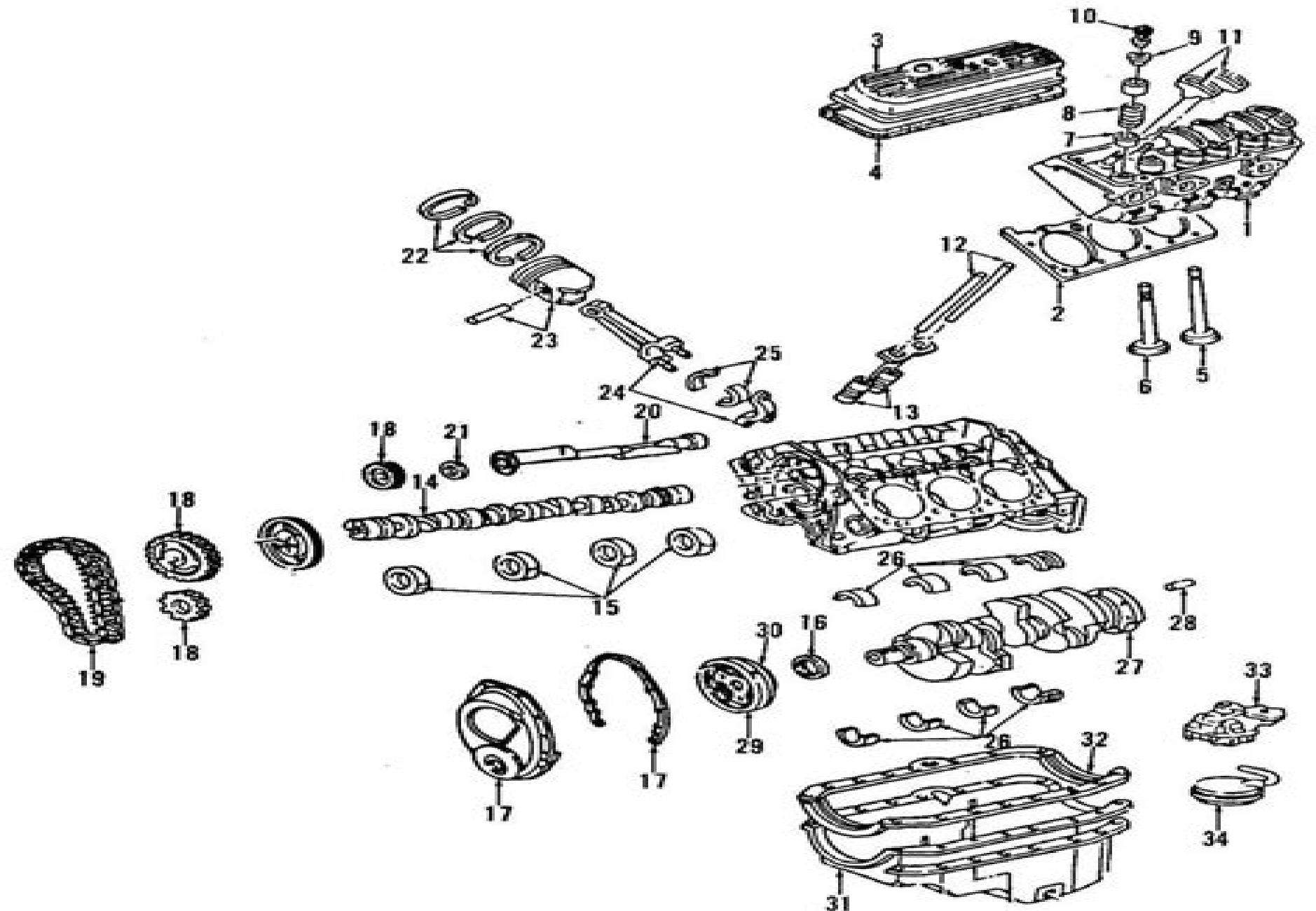
ENGINE - 4.3L W/ BALANCE SHAFT
