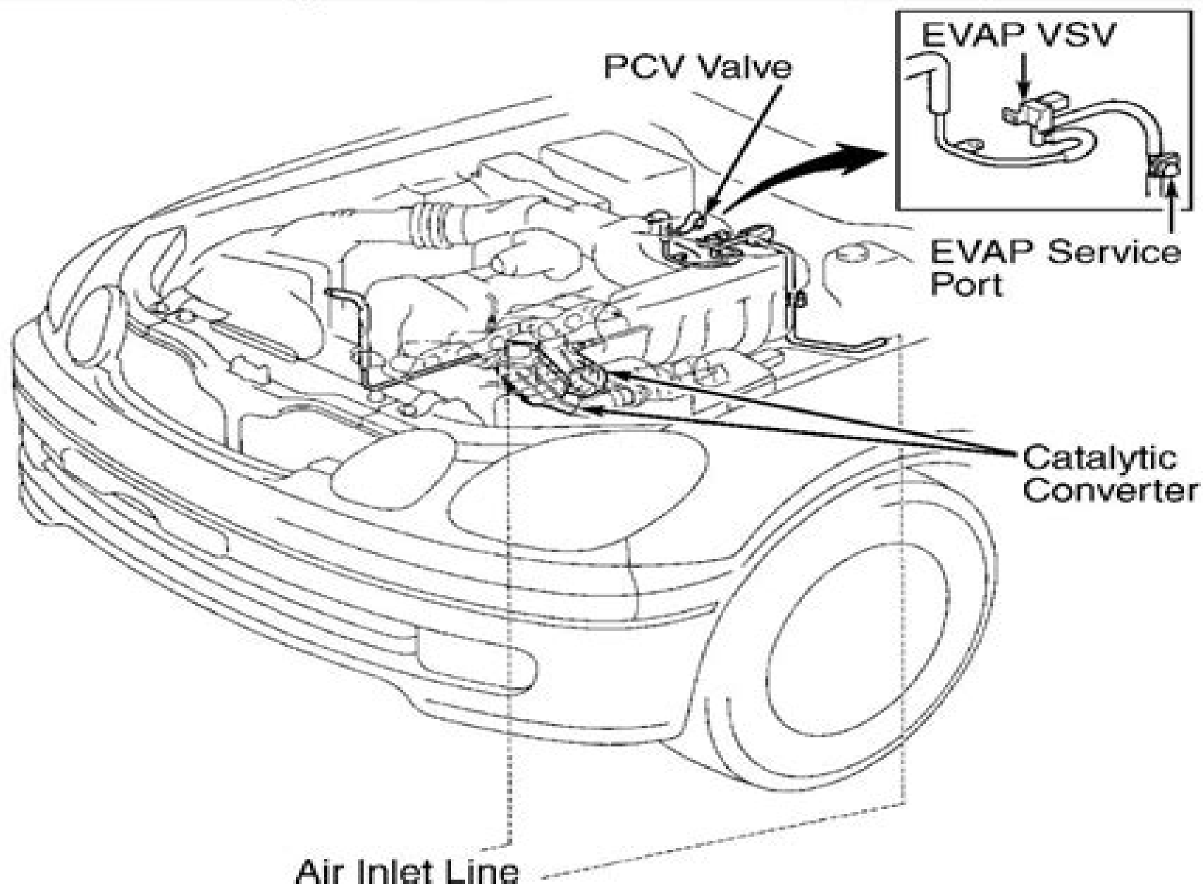
Fig. 5: Vacuum Diagram (GS300 - 1 Of 3)
