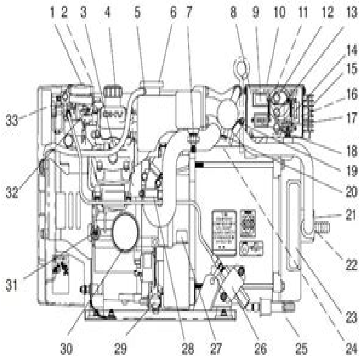
SERVICE VIEW
