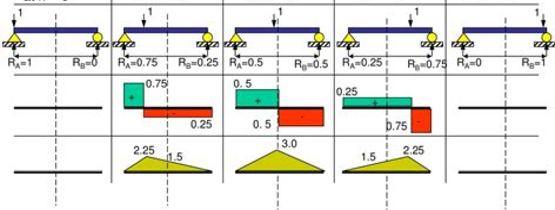
Unit load at x = 0
