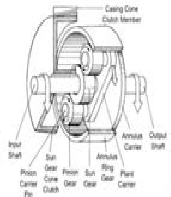
Epicyclic Gearbox
