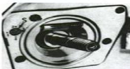
Fig. H41—View showing location of oil pump adjusting screw (S). Adjusting screw shown is set at position 2.
