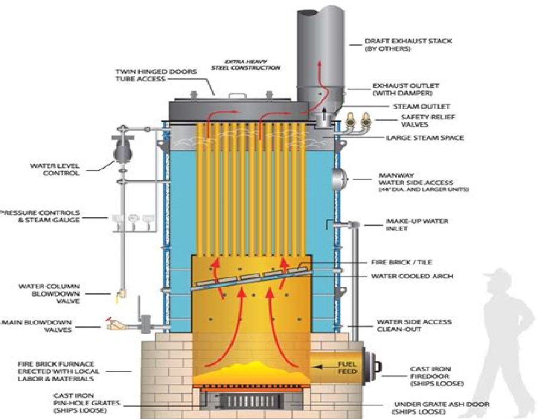
OPTIONAL ALL-STEEL FURNACE AVAILABLE
