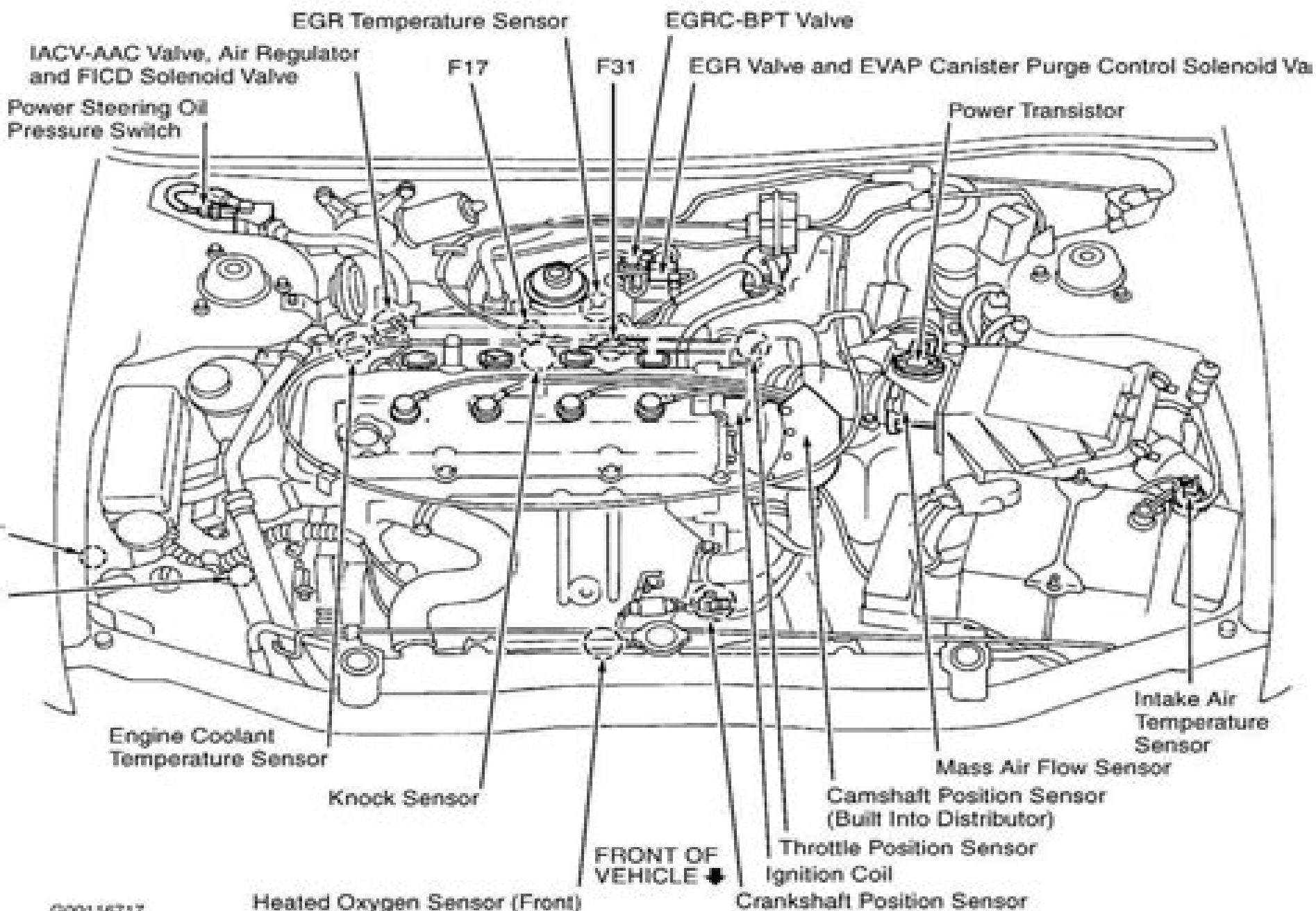
1997 Nissan Altima GLE Fig. 1: Engine Compartment
