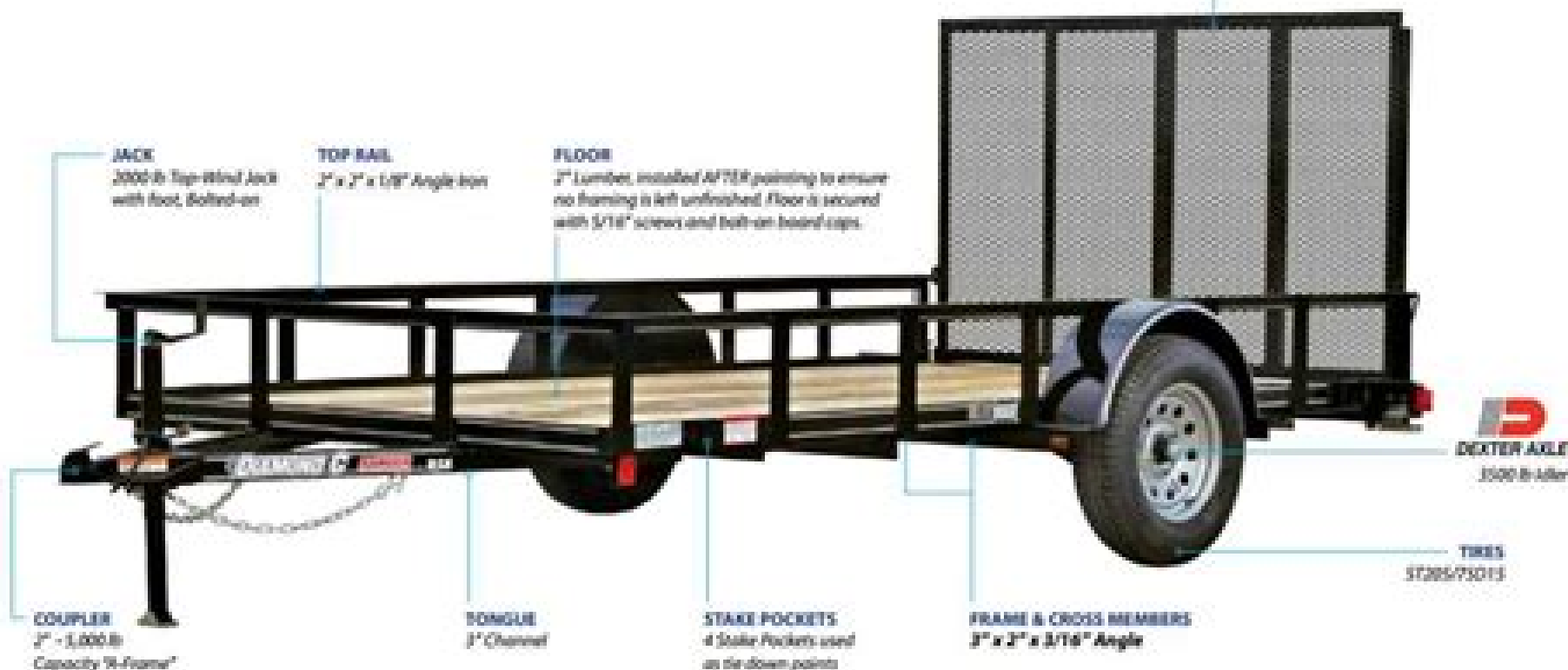
GATE OPTION Optional 48" Straight Ramp Gate Option folds flat on the trailer floor for storage
