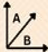
Complementary angle
