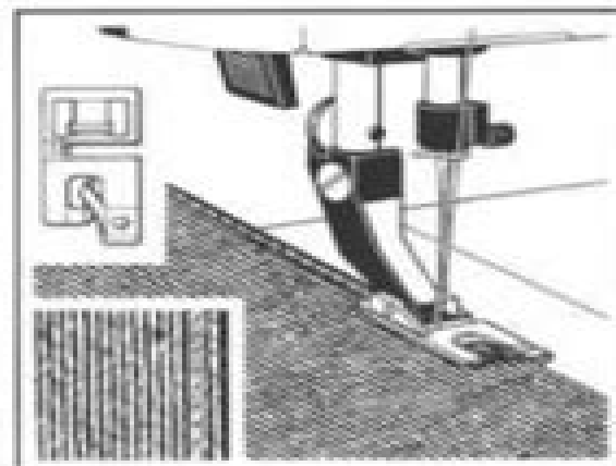
411 85 22-01. Presser foot for 2 mm hemming. For straight stitching or small zig-zag stitching, stitch length 1.5.
