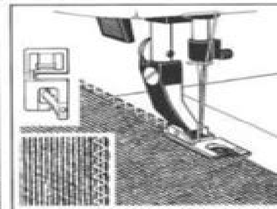
411 85 24-01. Presser foot for 2 mm rolled hem. For medium zig-zag stitching, stitch length 3. Suitable for light fabrics.
