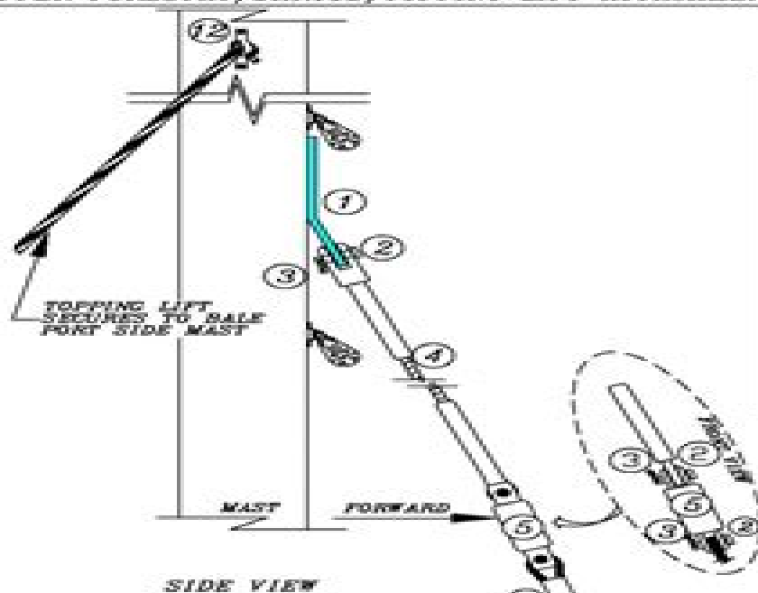
SIDE VIEW
