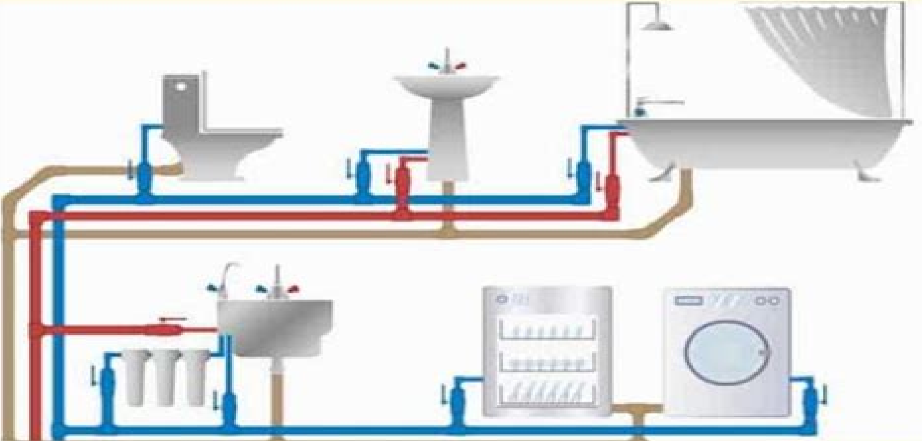
HOUSE PLUMBING SYSTEM DIAGRAM
