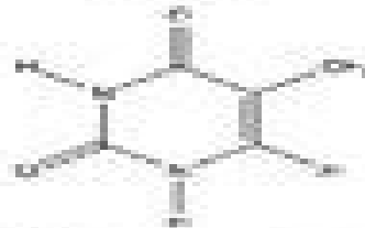
Thymine
