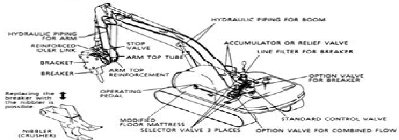
Fig. 1-2 Outside view of nibbler & breaker-attached machine
