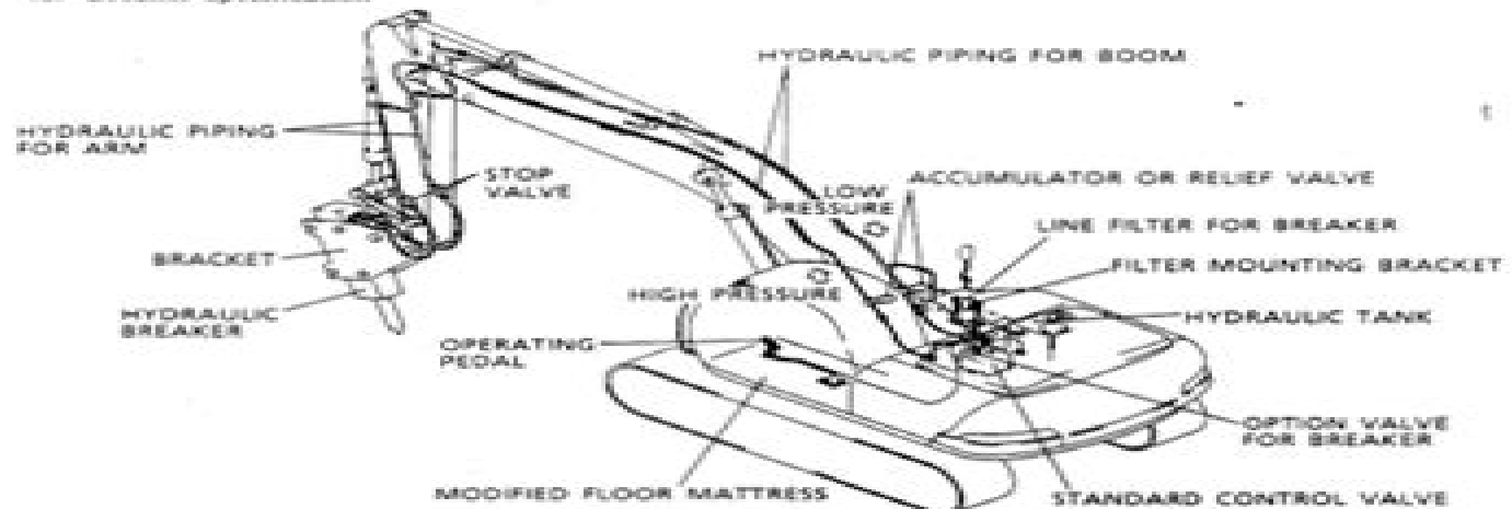
Fig. 1-1 Outside view of breaker-attached machine
