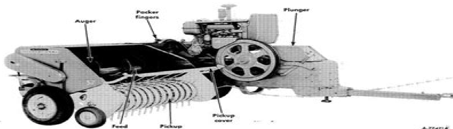
Illustr. 2 Right front view of the 57 Baler.
