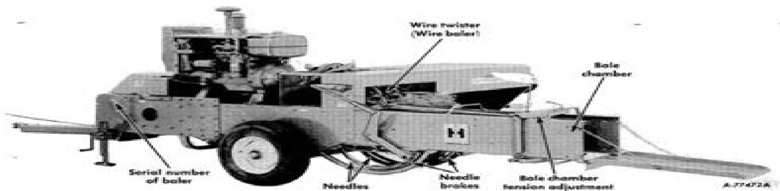
Illustr. 2A Left rear view of the 57 Baler.
