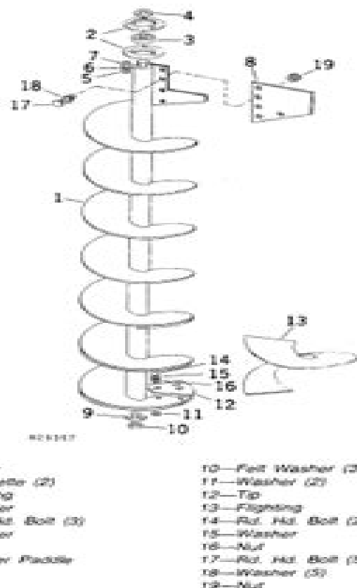
Fig. 4-Auger Components
