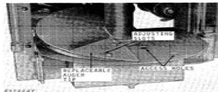
Fig. 5-Replacing Auger Tip
