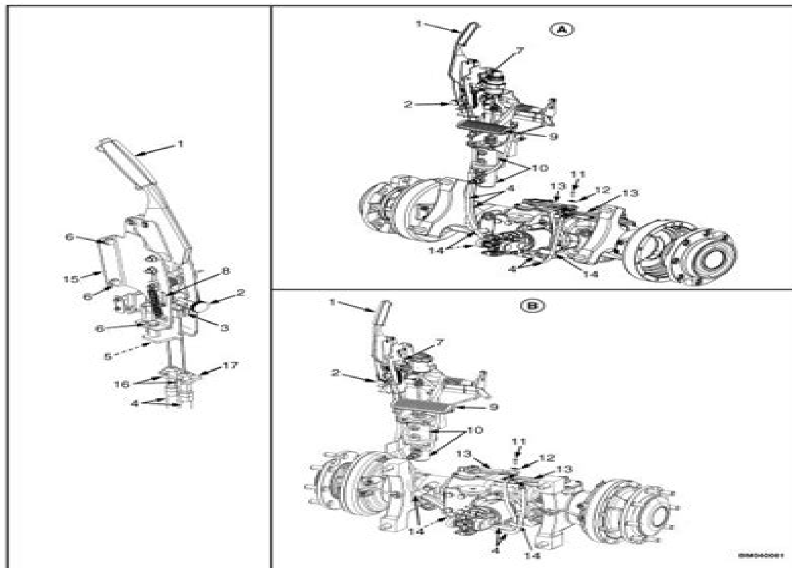
Figure 14. Parking Brake Lever Adjustment for Lift Truck Models S4.0, 4.5, 5.5FT, S5.5FTS (S80, 100, 120FT; S80, 100FTBCS; S120FTS; S120FTPRS) (G004) and H4.6FT5/FT6; H4.5FTS5, H4.5FT6; H5.0-5.5FT (H80, 90, 100, 120FT) (N005, P005) With Wet Brake System
