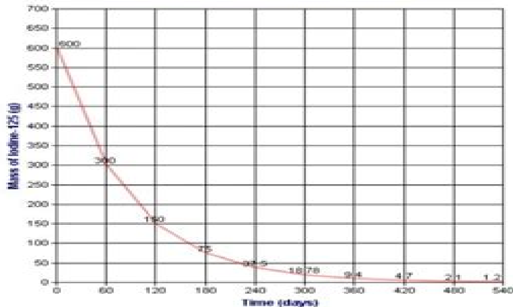
Radioactive Decay of Iodine-125
