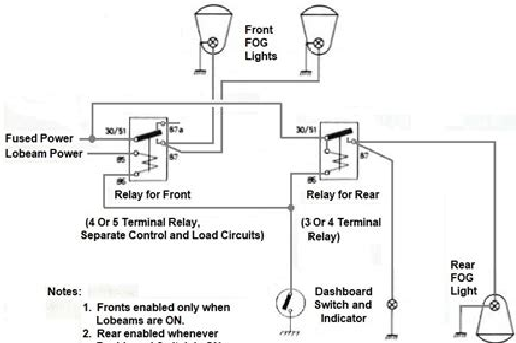
Fog-Light Control Wiring including Automated Control 24 Dec 2010 R. Kwas
