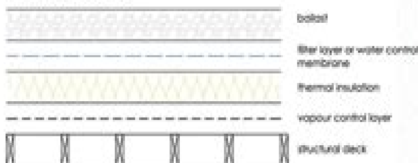
Inverted Warm Deck Roof
