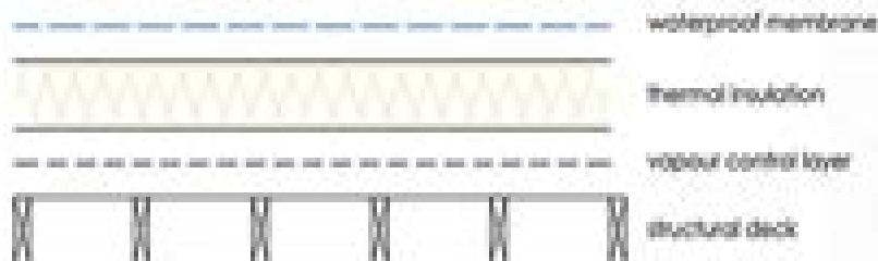
Warm Deck Roof
