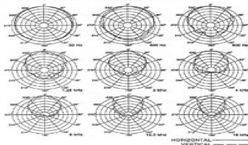
FIGURE 3 — Sx200 Beamwidth Response (anechoic environment)
