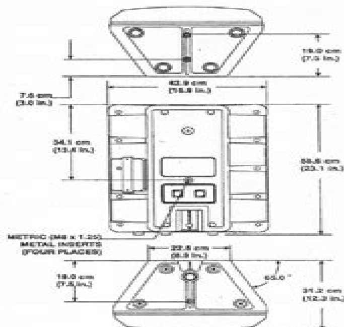
FIGURE 6 — Two-Conductor Cable Configurations for Sx200 Speaker System Using Neutrik Speakon® NL4FC Four-Pin Connector
