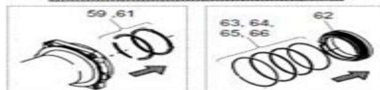
Fig. 34-26 Removing brake piston (62)
