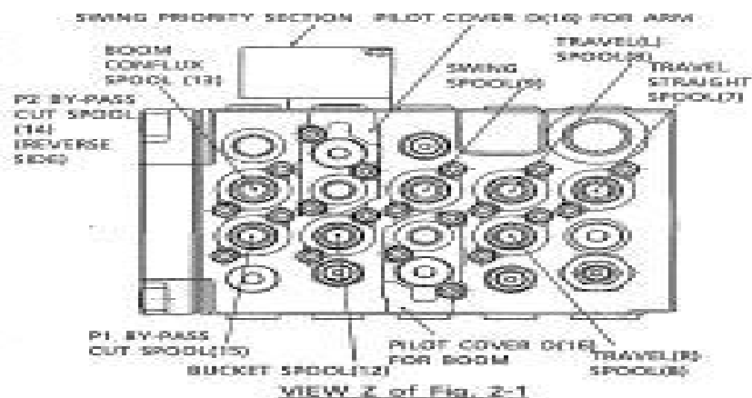
Fig. 2-2 Position of spool without lock valve
