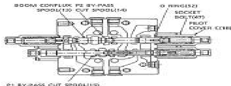
Fig. 2-4 Pulling out P2 by-pass cut spool, P1 by-pass cut spool and boom conflux spool (section EE)
