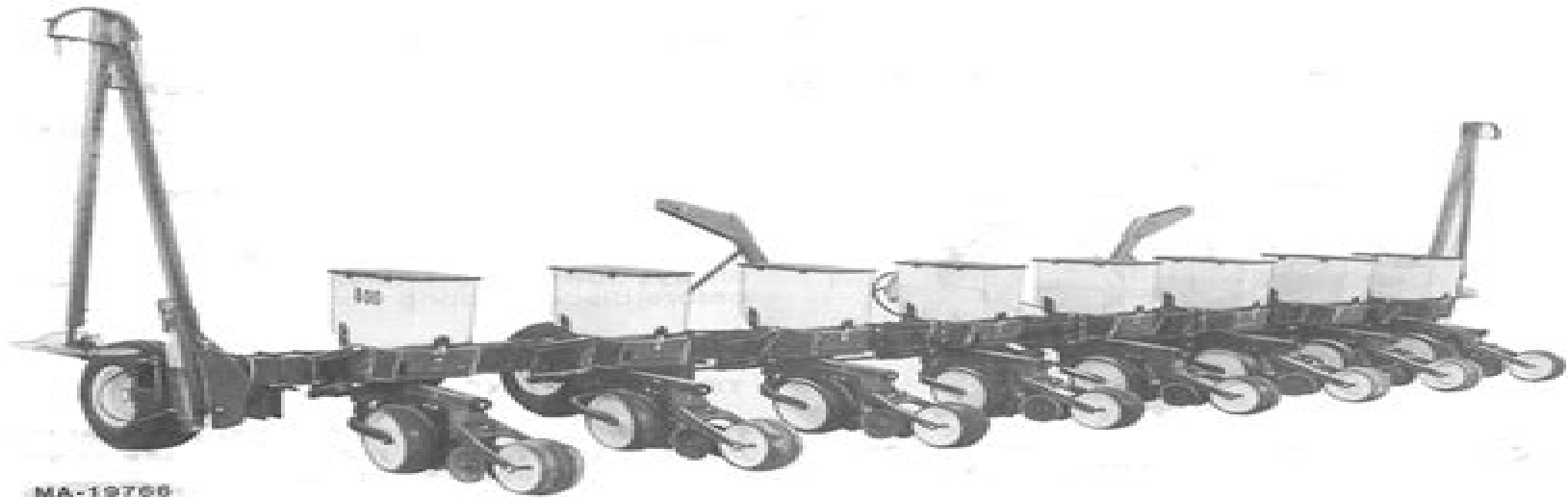
Eight row planter.
